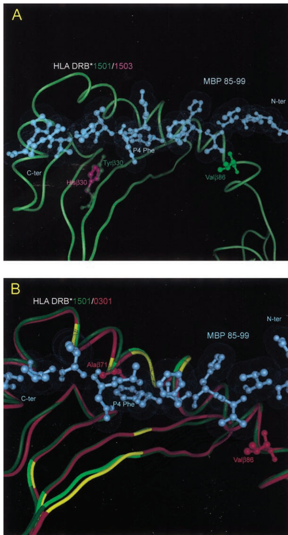
Figure 1 Molecular structures of MS-prone HLA-DR \beta 1 alleles. A , HLA-DR \beta 1*1501 and -DR \beta 1*1503 allelic structure are superimposed using MINRMS, a program for finding minimal root mean squared distance alignments between two proteins as a function of the number of matching residue pairs within a heuristically limited search space. The resulting structures were displayed as rods through use of Chimera (UCSF Chimera Home Page), an interactive molecular graphics program (Chiang et al. 2003). The structure of DR \beta *1503 was developed from the DR \beta *1501 crystal structure (Protein Data Bank [PDB] ID 1BX2) by mutating the residue at position 30 from Tyr to His, using the software Swiss PDB-viewer. The distinctive residues at position 30—Tyr for *1501 and His for *1503—are shown in green and magenta, respectively. Polymorphic residue Val \beta 86 (critical for the hydrophobic pocket characteristic of DR2 and DR3 alleles) is shown in green. MBP peptide 85-99 and its electronic cloud are shown in gray. B , HLA-DR \beta 1*1501 (green) is superimposed on DR \beta 1*0301 (PDB ID 1A6A; red) in a top view, and their differences are highlighted in dark green and yellow, respectively. Most of the allele-specific residues are in close proximity to the peptide and thus likely affect the MBP binding affinity. Residue DR \beta 1*0301Val 86 is shown in red. Residue labels are colored according to that of their respective molecule. For clarity, the DR \alpha chain was omitted in these representations.
